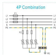
4P Combination
